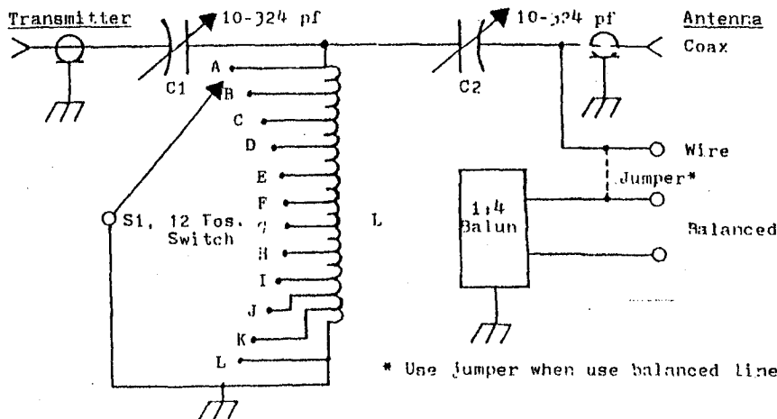
MFJ-901B Circuit Diagram
