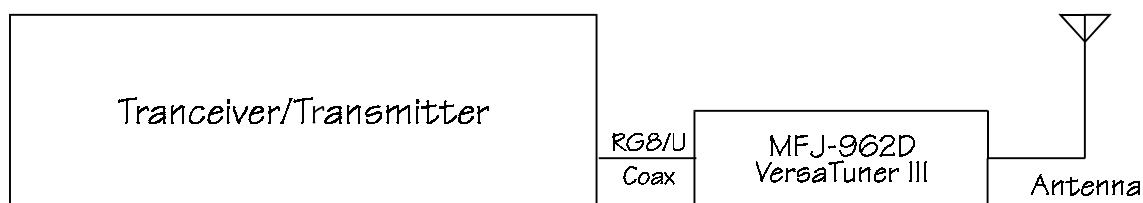
Block Diagram Figure 1
